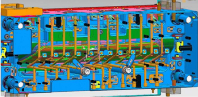
Cavity cooling system
